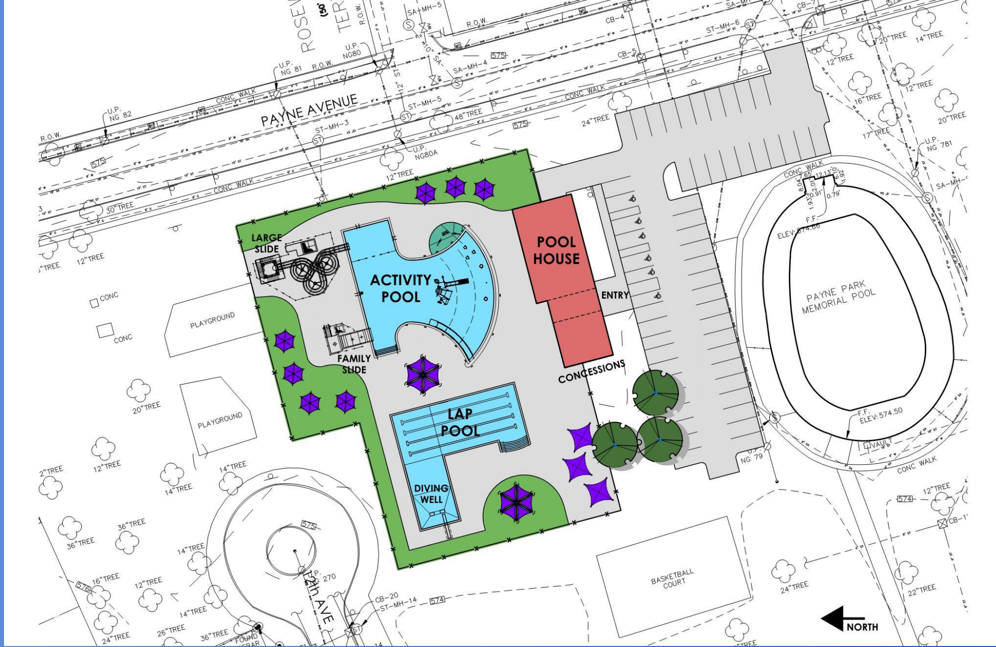
Pool Site Layout
